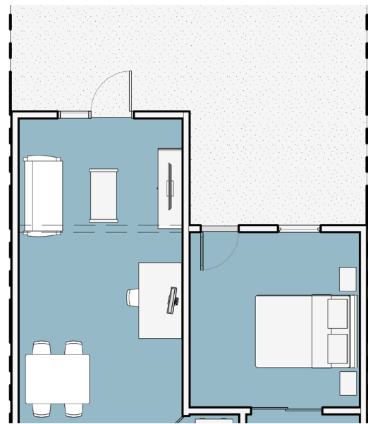
Variation of the ADU Plan for Prototype D, showing an extension into the rear yard.
