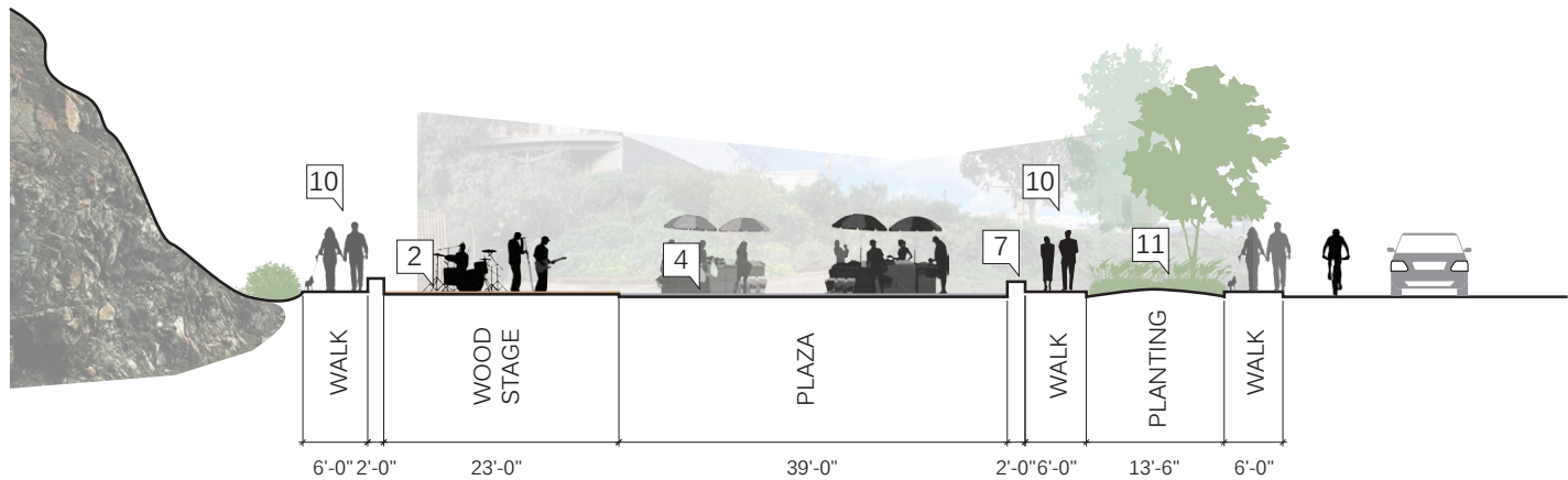
SECTION B-B
