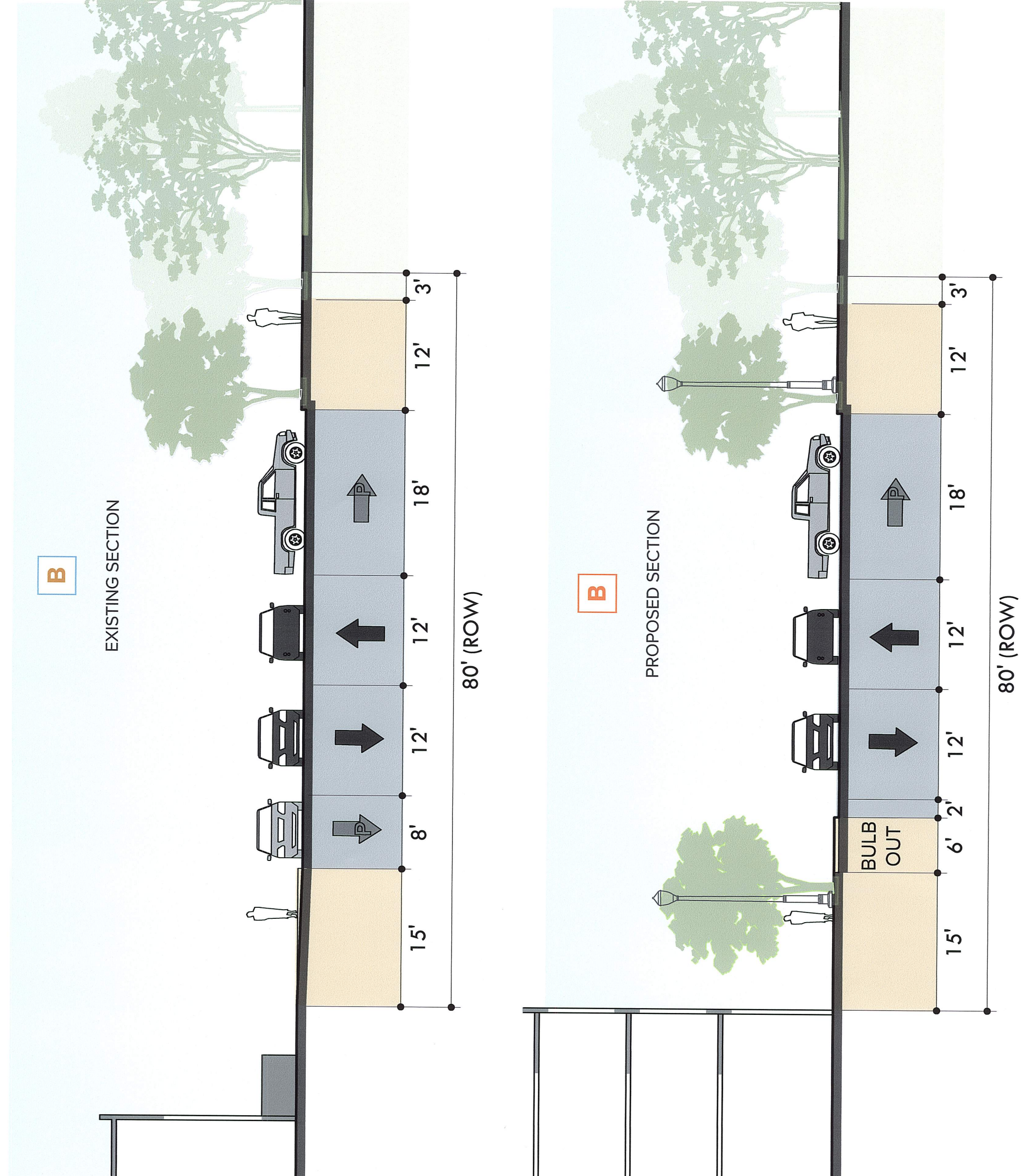
Section B (1"=10')
