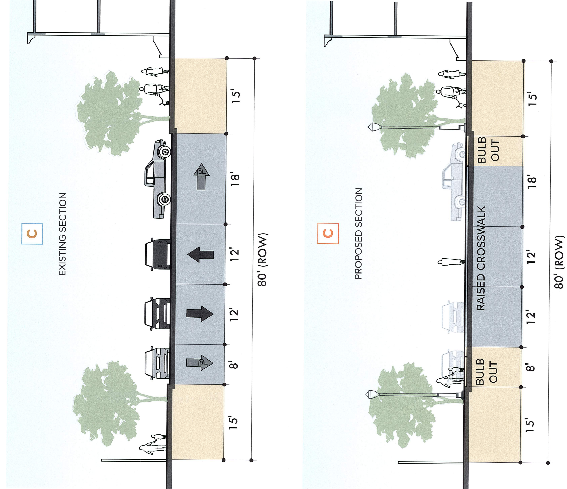
Section C (1"=10')
