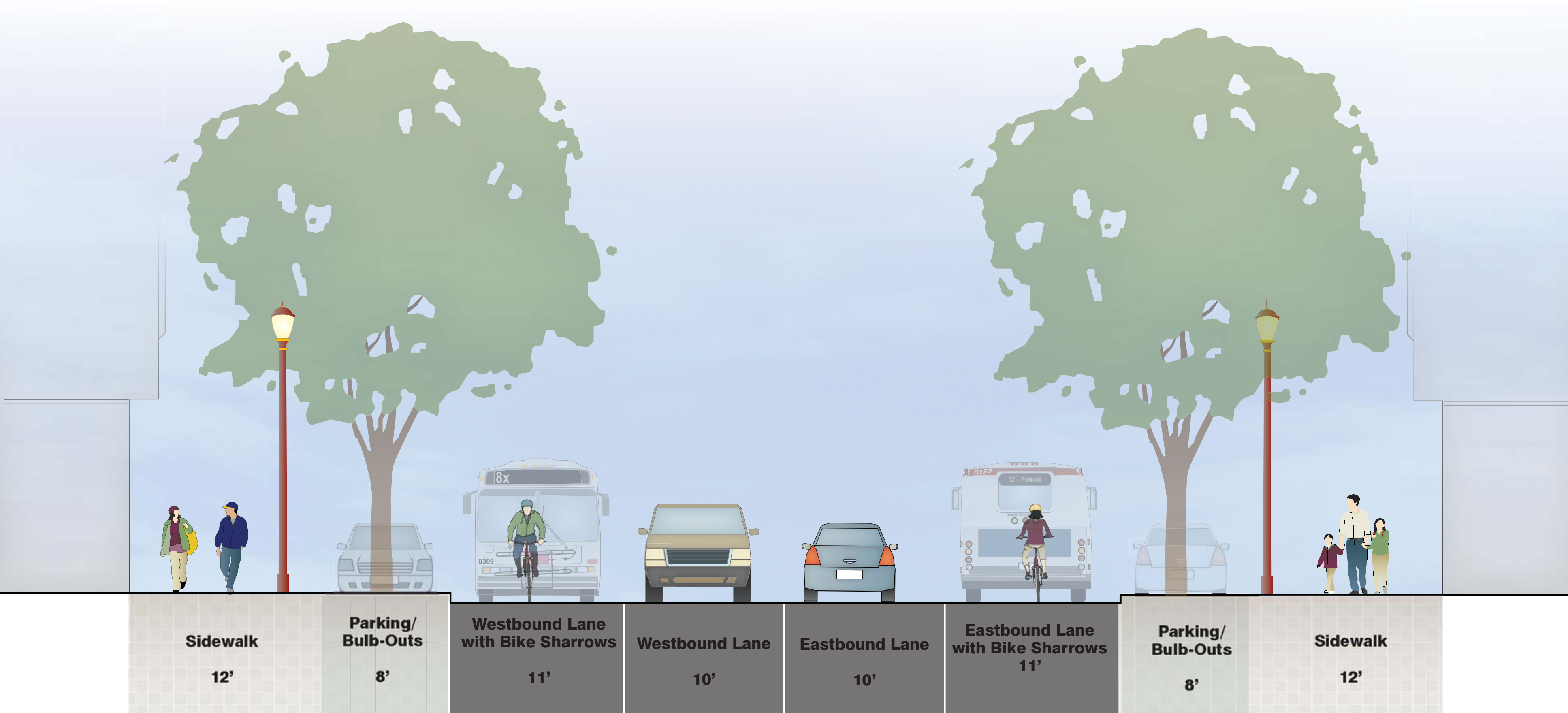
TYPICAL BROADWAY STREET SECTION NEAR INTERSECTION, LOOKING EAST: 向東面看 (即海灣大橋), 一般百老匯街的截面圖:
