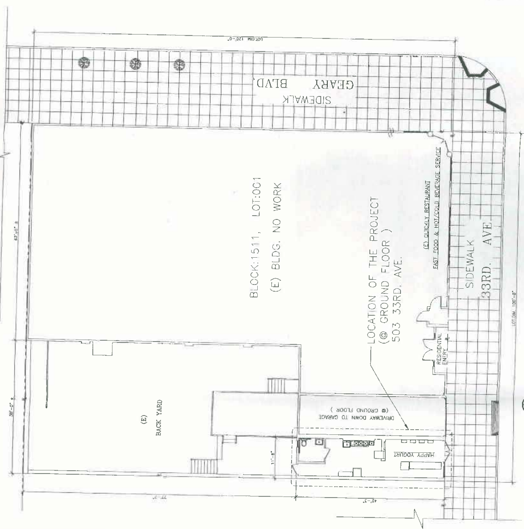
PROJECT SITE PLAN SCALE: 1/8"=1'-0" (6" GROUND FLOOR) SCALE IN FEET
