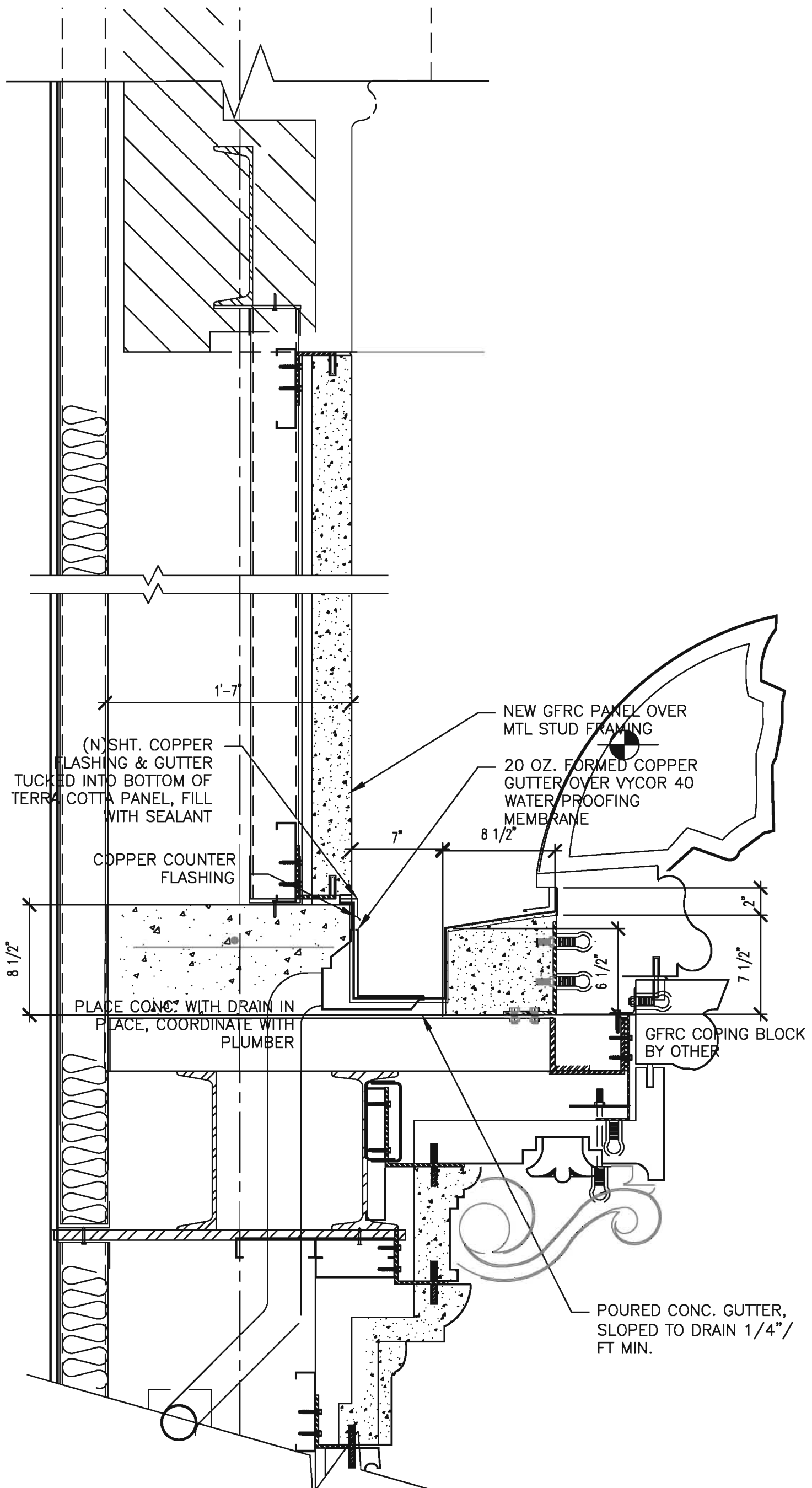
6 GUTTER & FLASHING AT WALL A1.1 1-1/2" = 1'-0"
