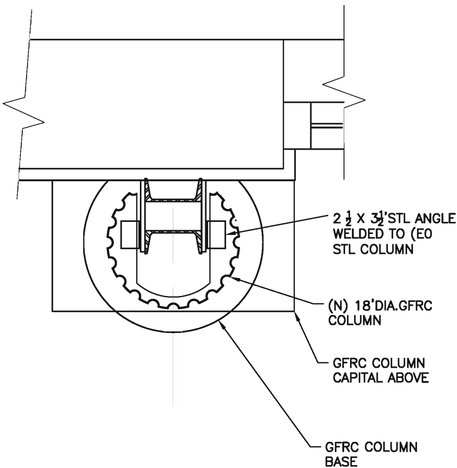
2 GFRc COULUMN ATTACHMENT A1.1 1" = 1'-0"
