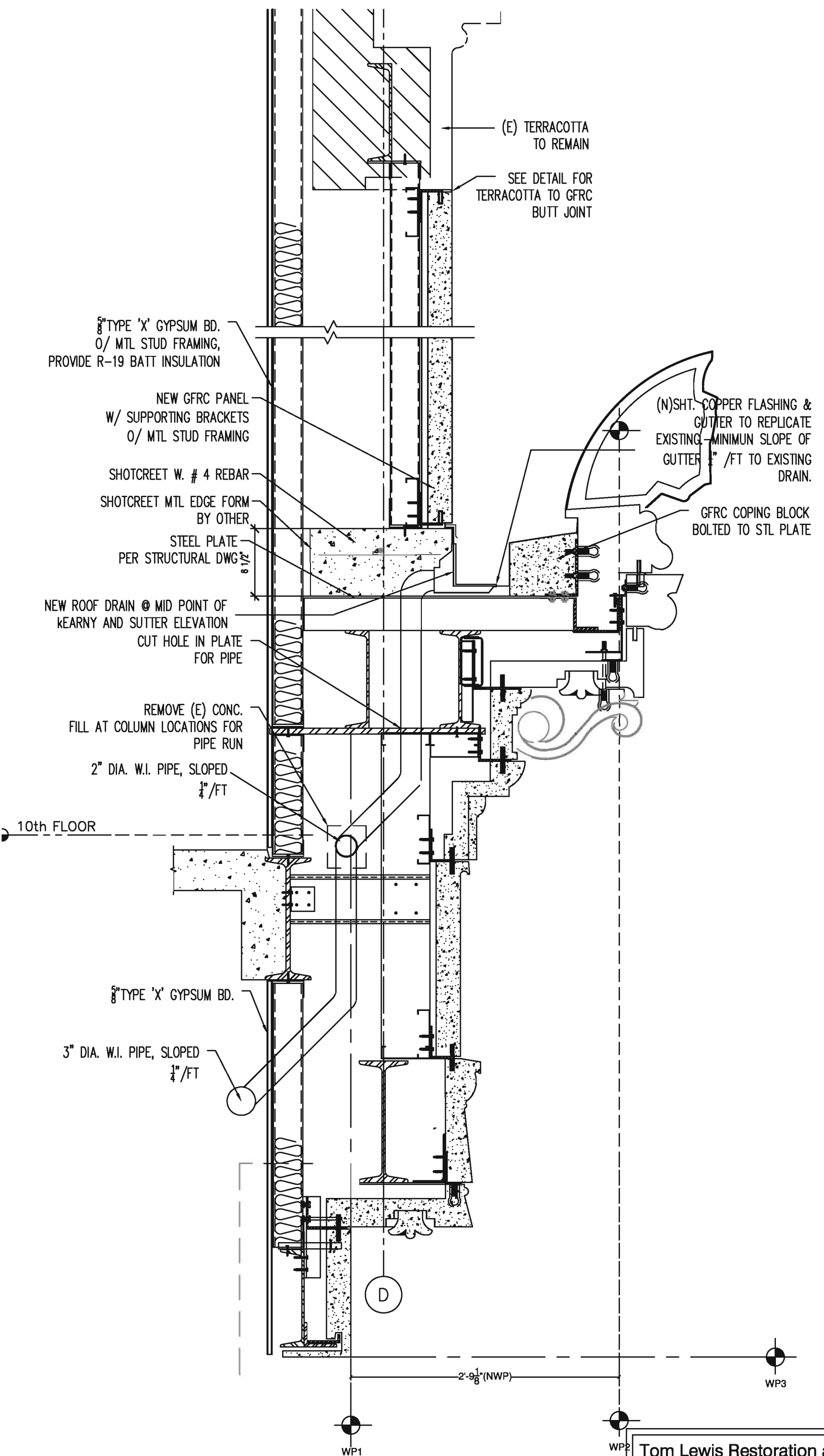
1 GFRC WALL SECTION—KEARNY ST. A1.1 WALL SECTION BETWEEN WINDOWS SIMILAR AT SUTTER ST. 1" = 1'-0"
