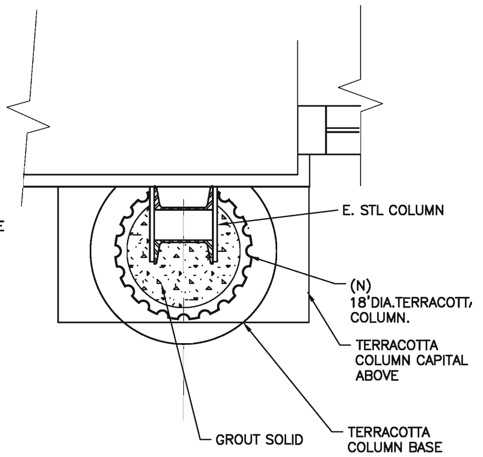
1 TERRACOTTA COLUMN SECTION A1.1 1" = 1'-0"
