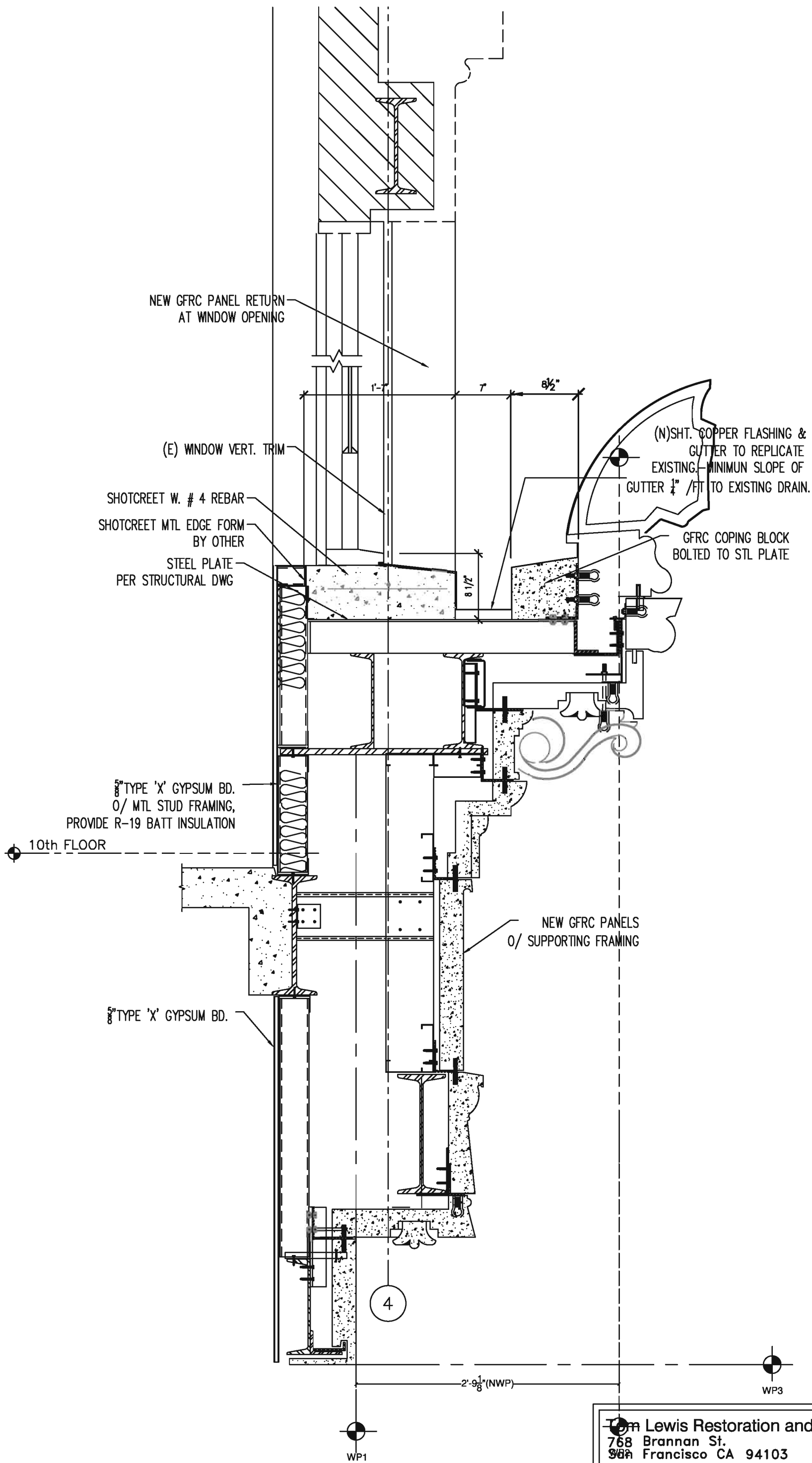
1 GFRC, GUTTER DETAIL-SUTTER ST. A1.1 WINDOW/GUTTER SECTION SIMILAR AT KEARNY ST 1" = 1'-0"
