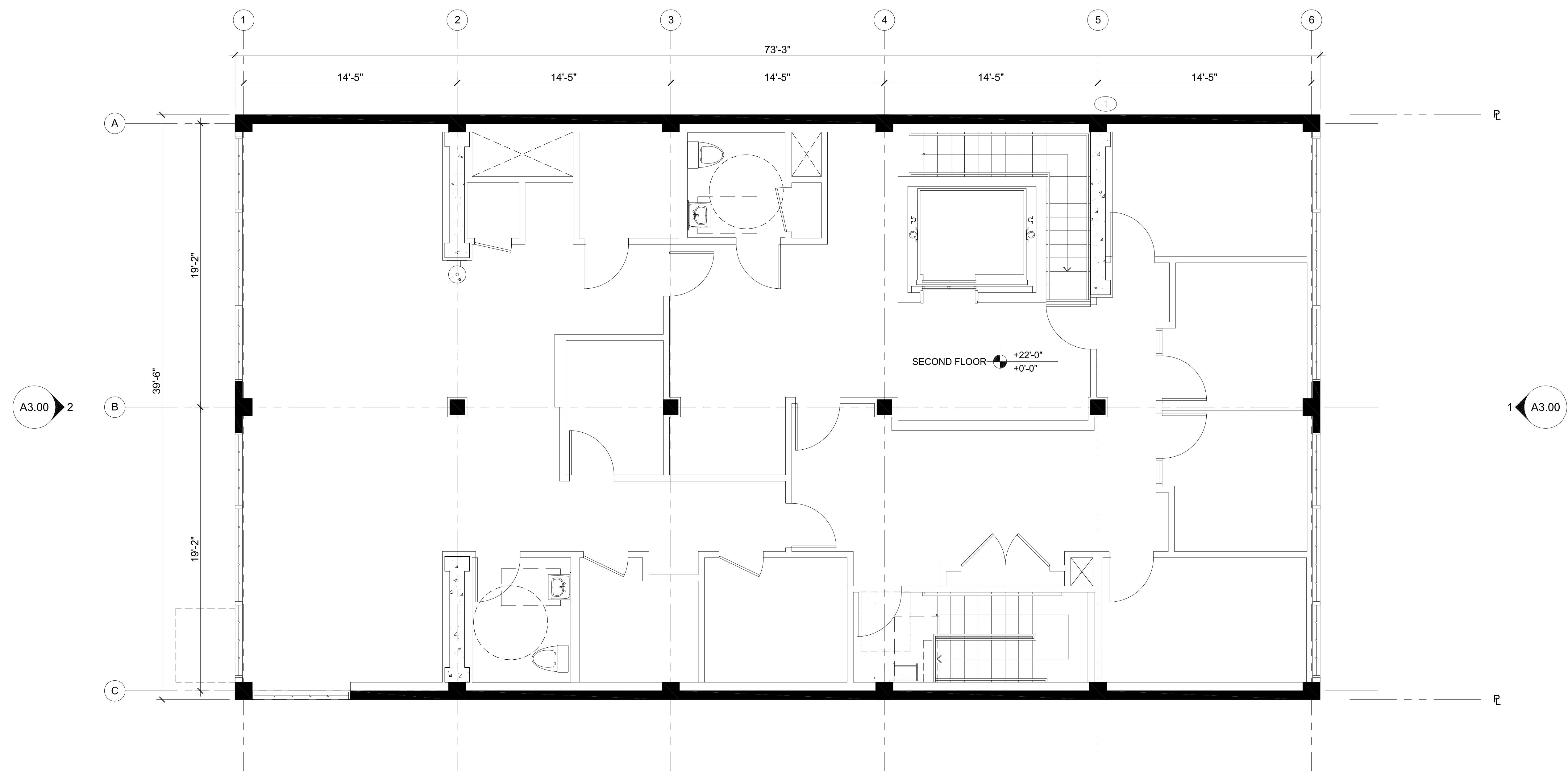
1 SECOND LEVEL FLOOR PLAN 1/4" = 1' - 0"
