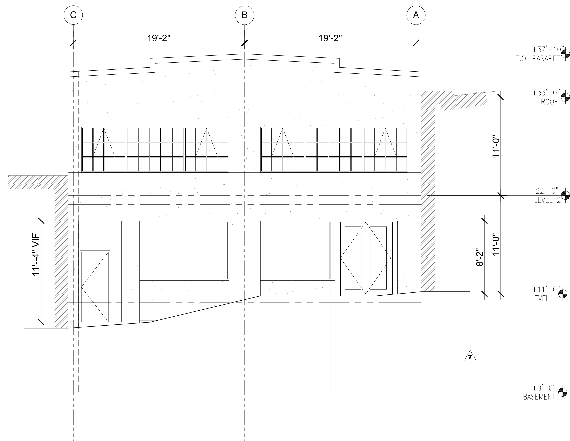
3 PROPOSED PACIFIC AVE. ELEVATION 3/16" = 1' - 0"
