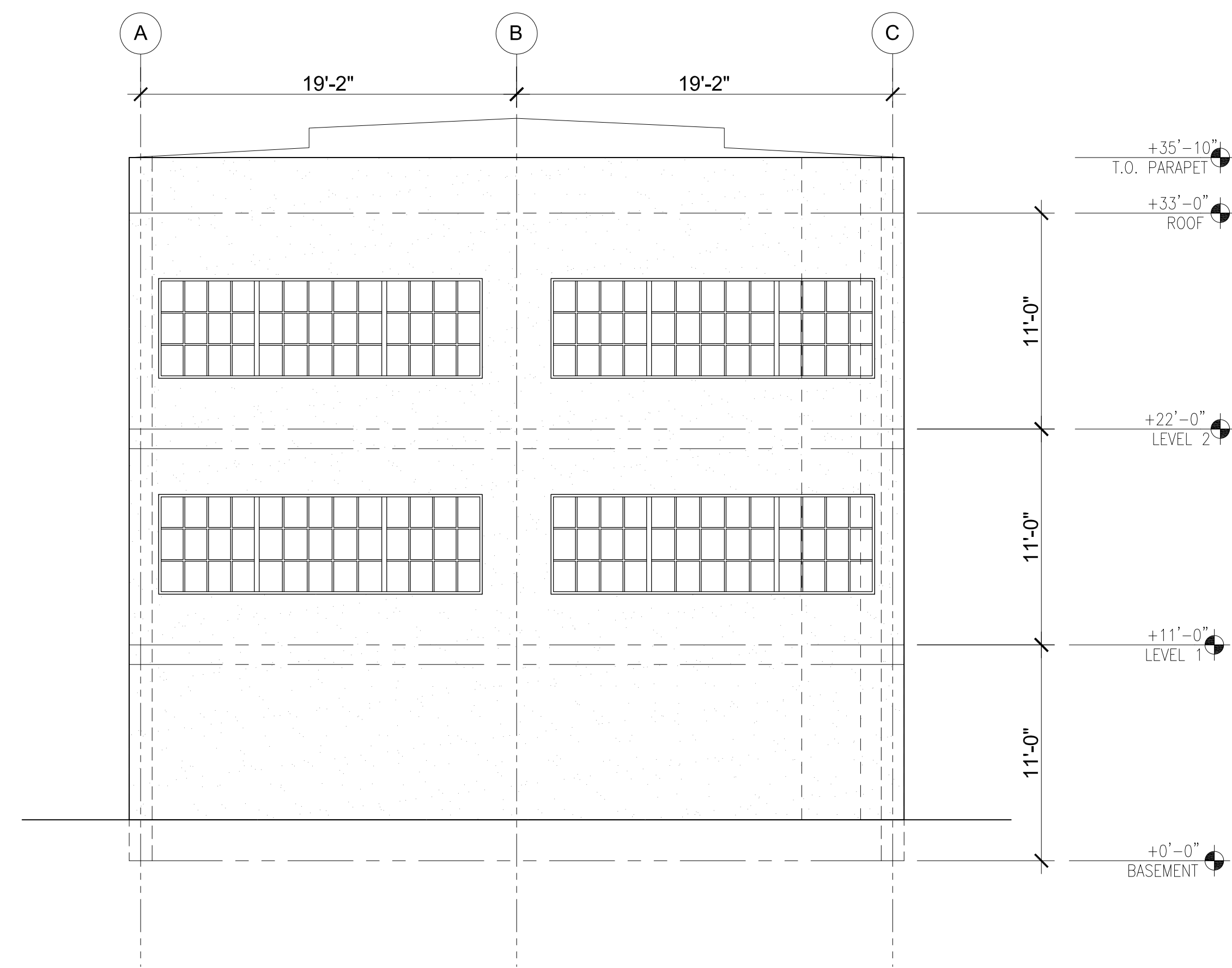
4 PROPOSED ALLEY ELEVATION 3/16" = 1' - 0"
