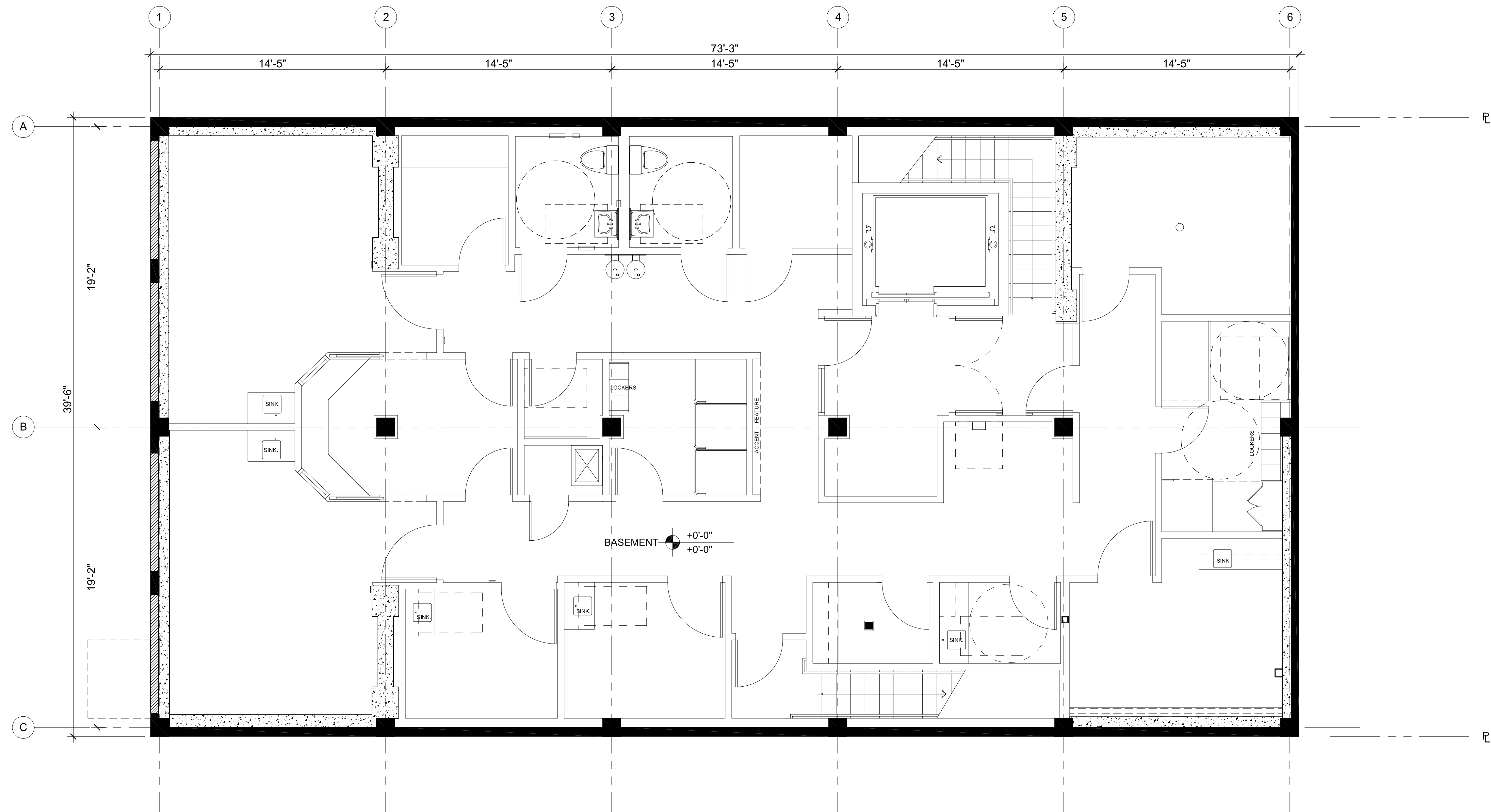
1 BASEMENT FLOOR PLAN 1/4" = 1' - 0"
