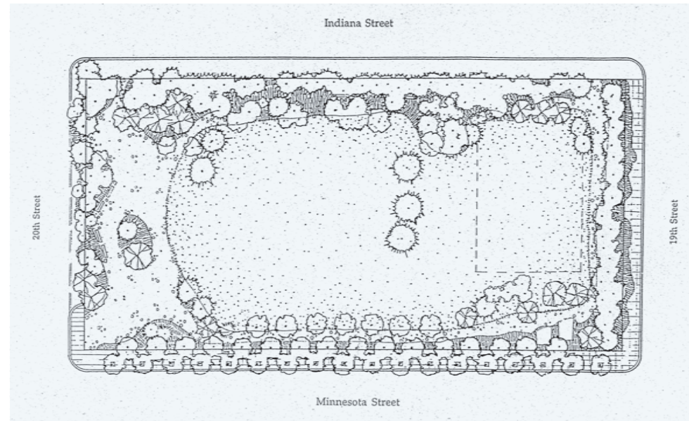
FIGURE A-97. ESPRIT PARK: ORIGINAL CONCEPT DESIGN BY ANDREW DETSCH
